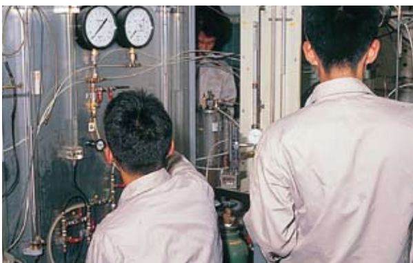
非排水状態下のしらすの三軸圧縮試験 Triaxial compression test for Shirusu under CU condition
