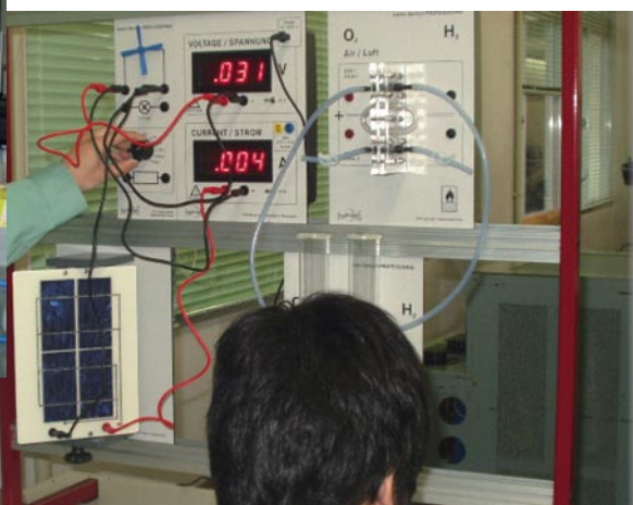
太陽電池と燃料電池特性実験 Characteristics of PV Cell and Fuel Cell
